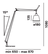
Tolomeo Basculante Reading floor
